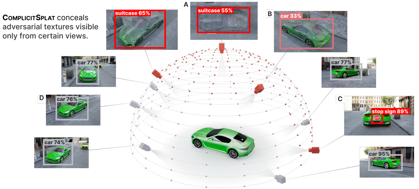
Fig. 1: COMPLICITSPAT conceals multiple adversarial cloaked textures in 3DGS scenes using Spherical Harmonics, causing the 3DGS representation of the car to become adversarial at different view points (red dots). For example, (A) when viewed from the top, the car appears as a suitcase, (B) “car” detection confidence decreases, (C) and when viewed directly from behind, displays a “stop sign.”
